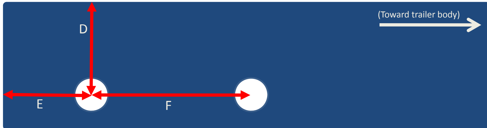
Side view of tongue with coupler removed
